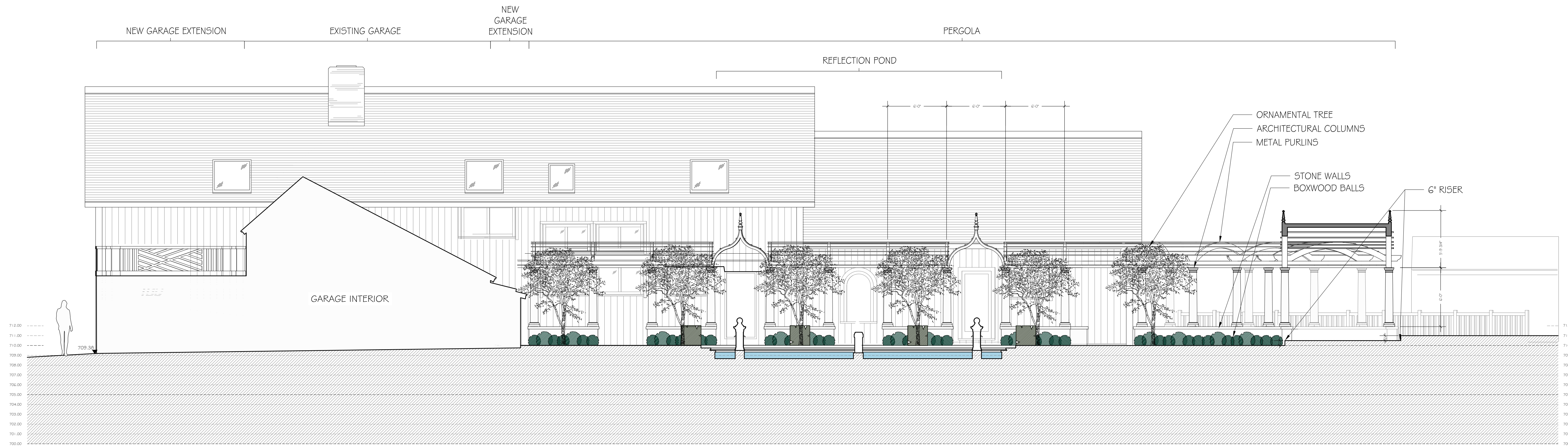
4 SECTION D-D' 3/16" = 1'-0"
