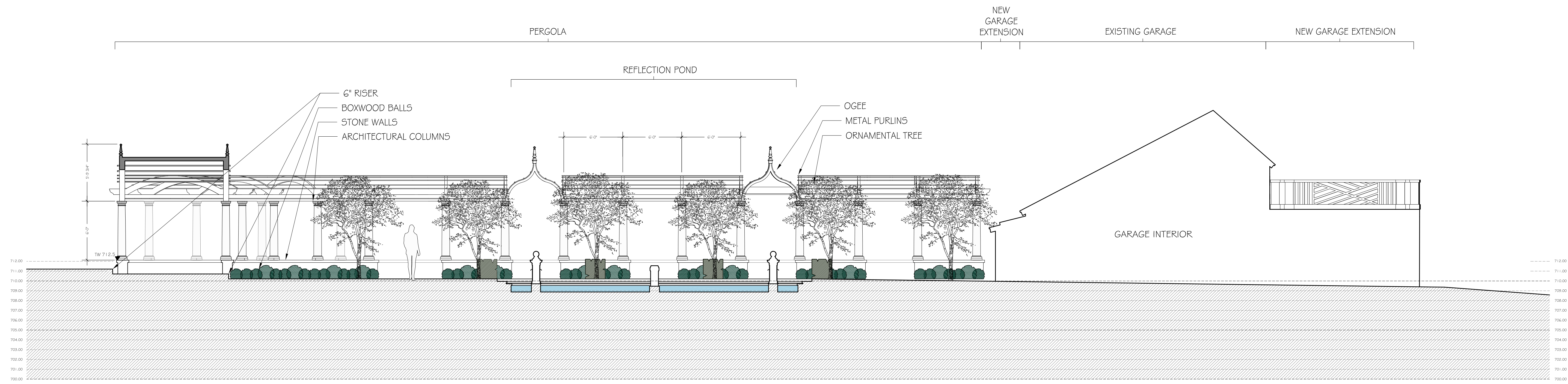
3 SECTION C-C' 3/16" = 1'-0"
